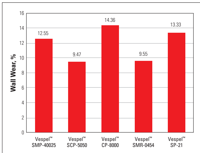
Figure 1. DuPont Vibratory Rig Wear; 475 °F/25 hr/55 lb
